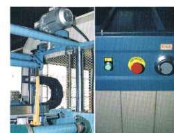
电动粘胶平台升降装置 Electronically controlled support table for pocket spring unit
