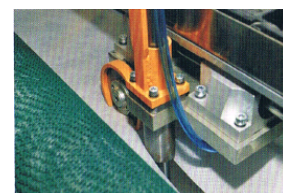
电动上下布裁切装置 Electronically controlled cutting device for the top&bottom fabric
